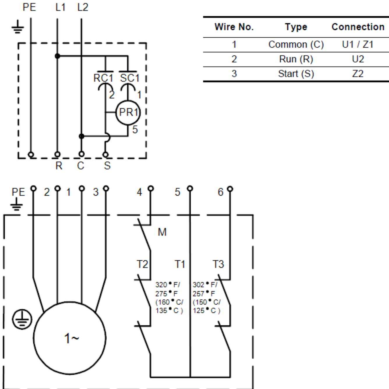
Fig. 1. Wiring Diagram, 1 phase 208-230, 60 Hz.
