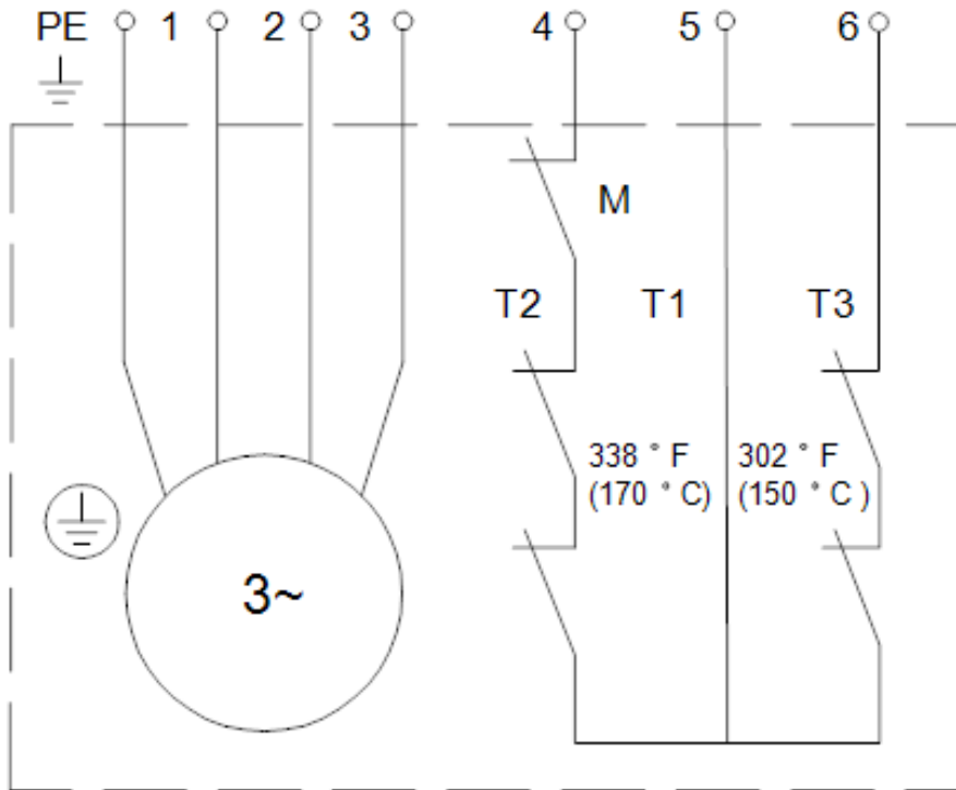
Fig. 2. Wiring Diagram, 3 phase 200-230/460, 60 Hz.
